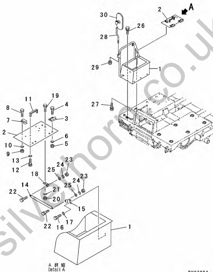
FIG.204 FRAME RELATED PARTS (4/4) (BATTERY BOX)
