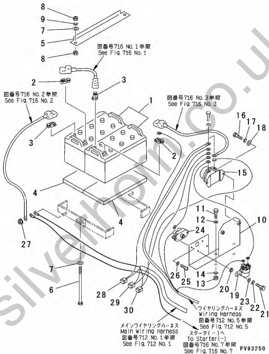
FIG.715 ELECTRICAL SYSTEM (3/4) (BATTERY AND BATTERY RELAY )
