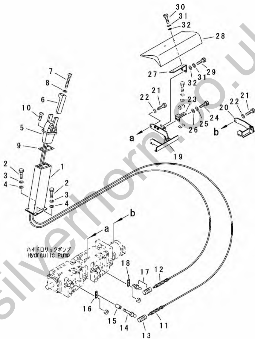
FIG.401 STEERING CONTROL SYSTEM
