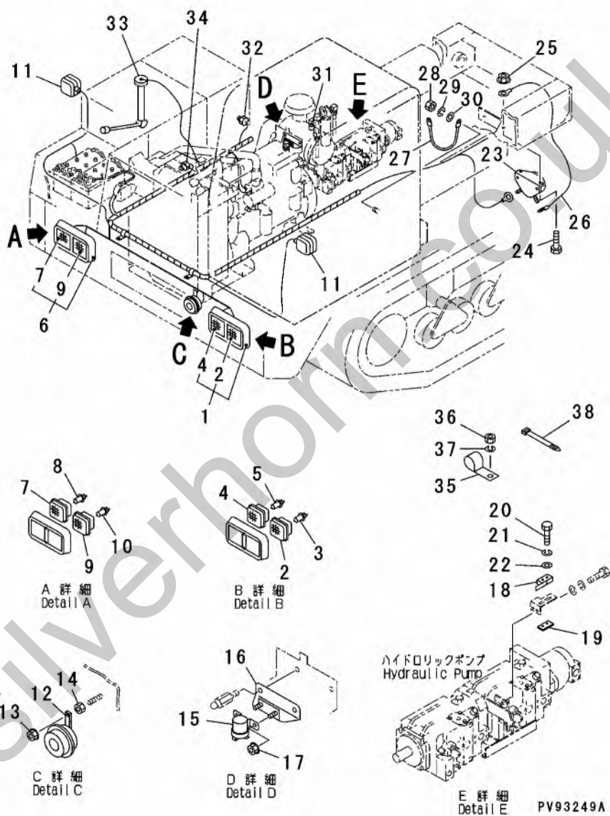
FIG.711 ELECTRICAL SYSTEM (1/4) (CHASSIS WIRING HARNESS AND LAMPS)
