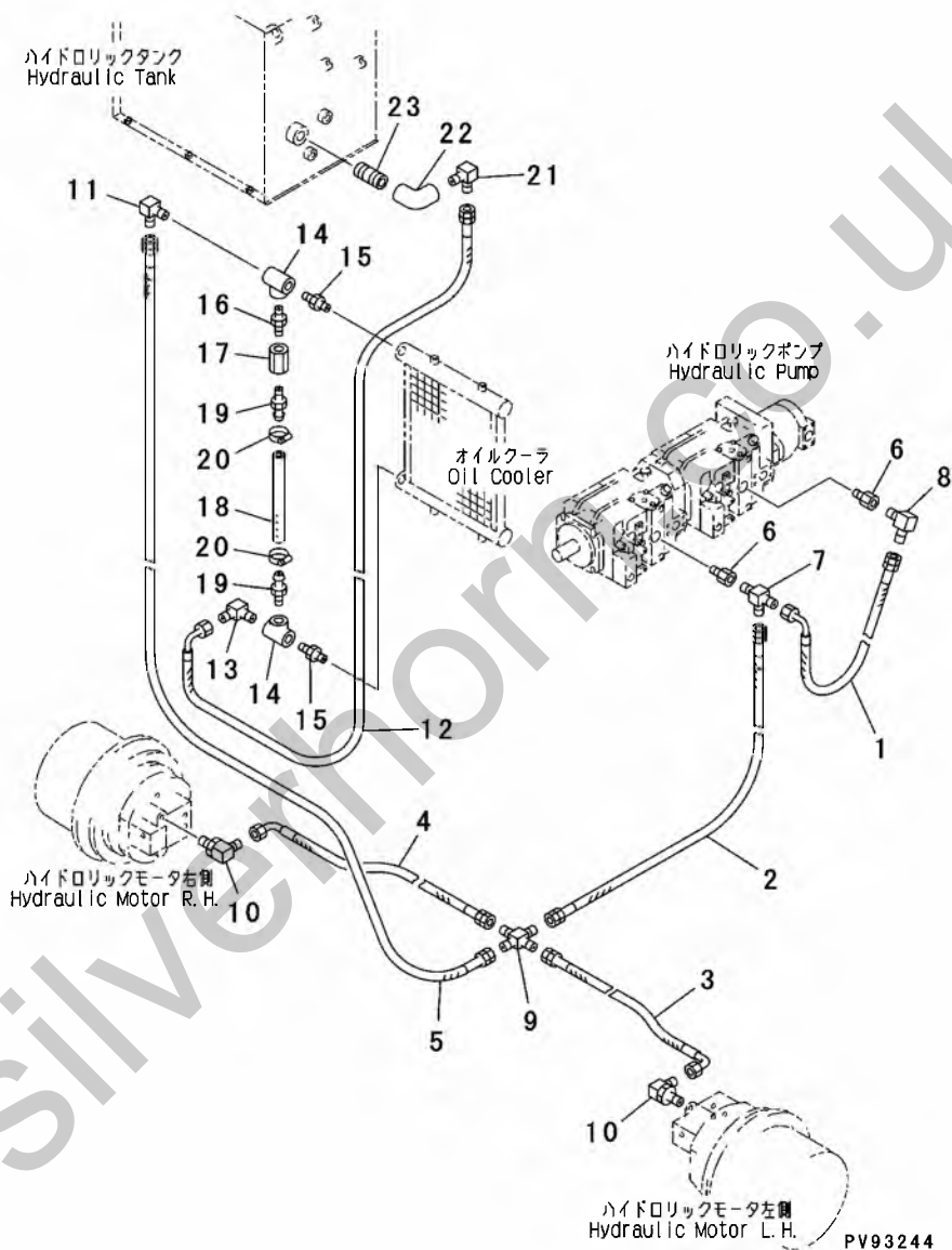
FIG.505 HYDRAULIC PIPING (OIL COOLER AND DRAIN LINE)
